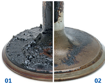
01 Baked-on deposits on inlet port valves can lead to sticking, incorrect sealing and reduced engine compression.
